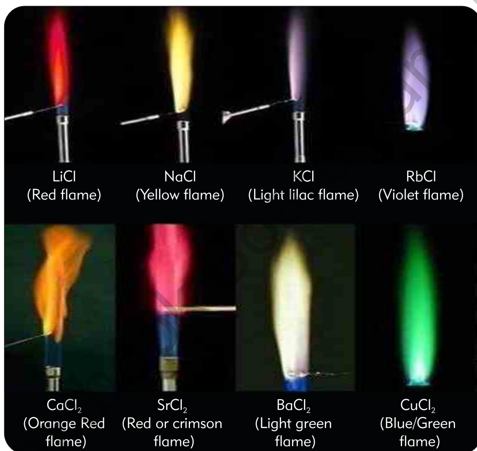
Figure 7.2 Flame test
