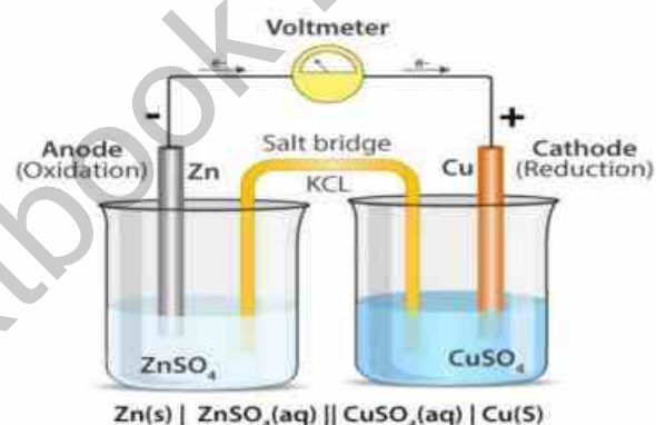
Figure 7.19 Electrochemical cell
