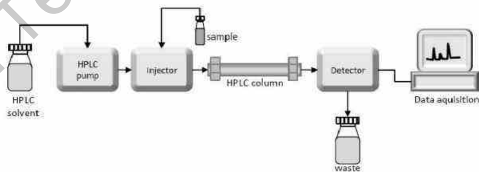
Figure 7.17 HPLC
